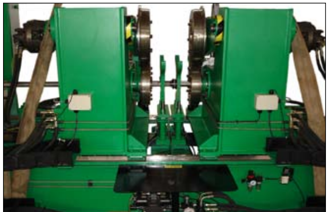
Rear view
