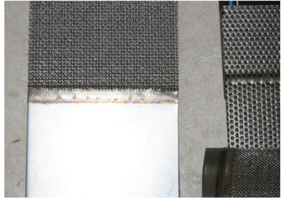
Examples of fully wetted filter material mesh to mesh and mesh to stainless steel sheet displayed in a rolled and flat condition.
